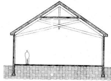
MEETING ROOM SECTION
